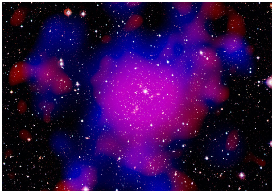
Components of the galaxy cluster Abell 2744, also known as the Pandora Cluster: galaxies (white), hot gas (red) and dark matter (blue). Credit: ESA/XMM-Newton (X-rays); ESO/WFI (optical); NASA/ESA & CFHT (dark matter)
